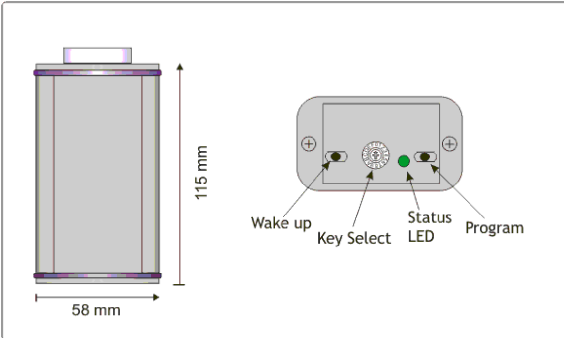
Dimensions & Interfaces of KeySafe
