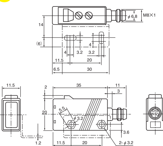
"-J" (M8 connector type) head-on model
