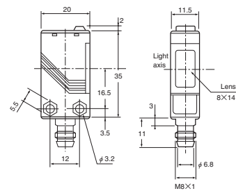
FBC-4R2S (Straight)
