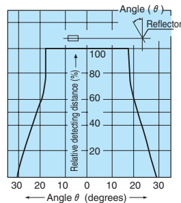
GMR2RSN · GMR2RN
