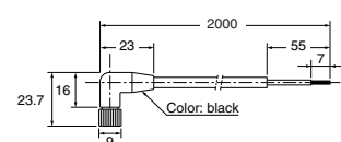
FBC-4R2L (Angled)
