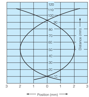
GR60R (50 x 50 White drawing paper)
