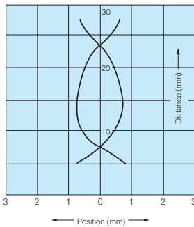
GR12RS • GR12R (50 x 50 White drawing paper)
