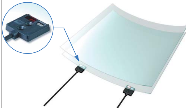
Optical system employing two LEDs as light sources. Used for reliable detection of inclined or warped glass.
