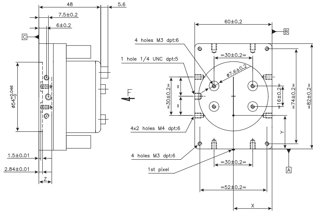
Figure 10-2. 6k Pixel Camera
