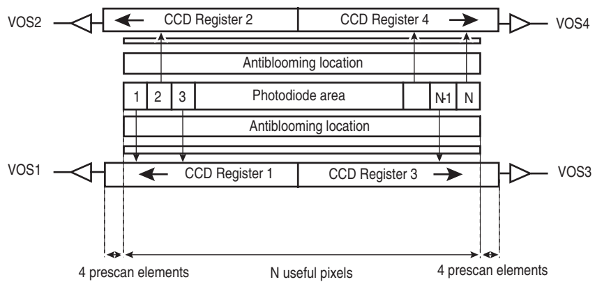
Figure 2-1. CCD Architecture
