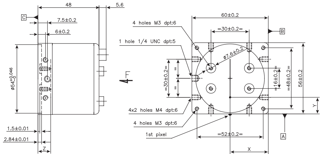
Figure 10-1. 2k Pixel Camera
