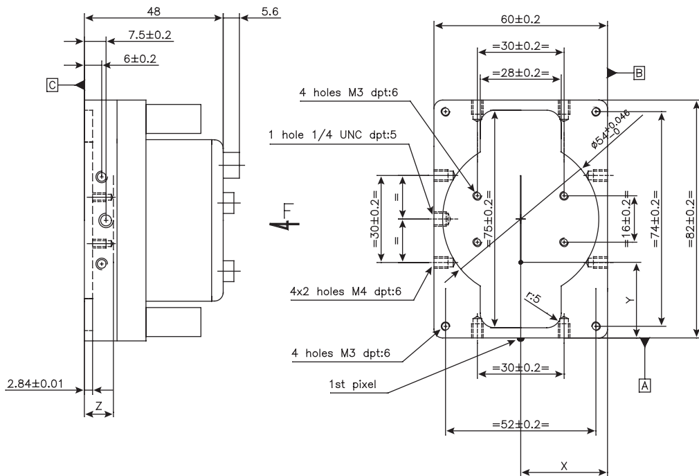
Figure 10-3. 8K Pixel Camera
