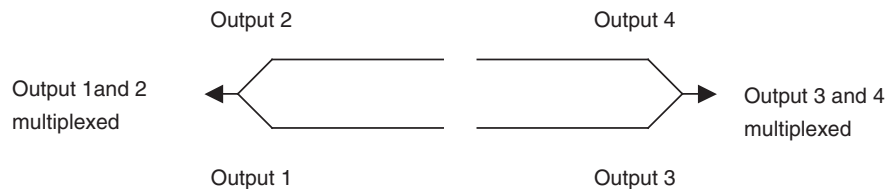
Figure 2-7. Camera Link Base Mode
