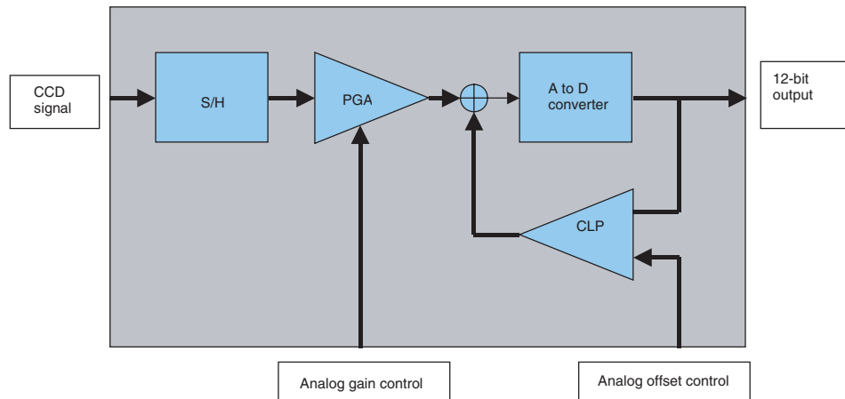
Figure 2-3. Analog Chain
