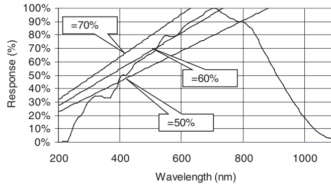
Figure 1-1. Spectral Response
