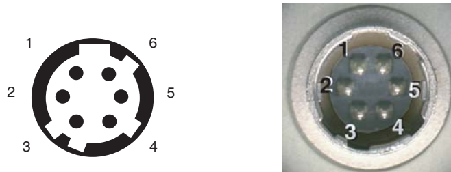
Figure 8-1. Receptacle Viewed from the Rear of the Camera
