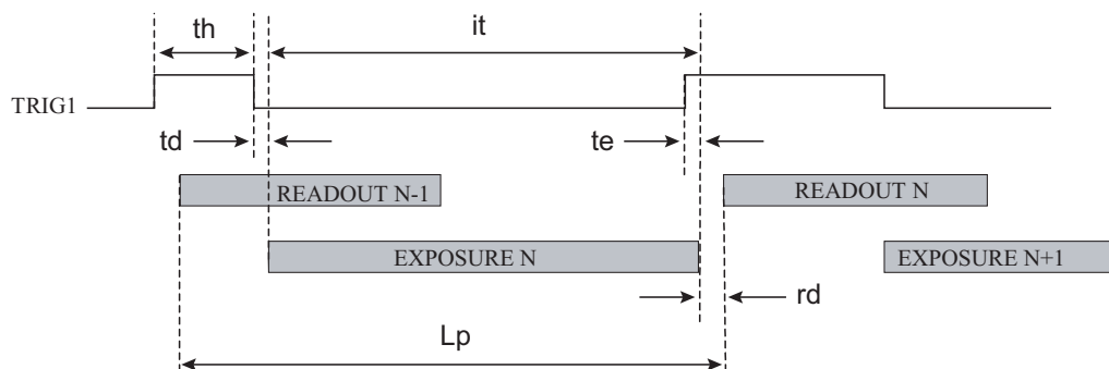
Figure 6-3. ITC Mode with One Signal Timing Diagram
