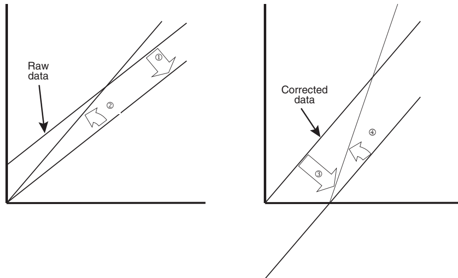
Figure 2-5. FCC and Contrast Expansion
